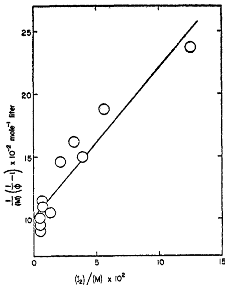
FIG. 1. Test of equation X for the photolysis of acetone in the presence of iodine at 3130 Å. and 100°C.
